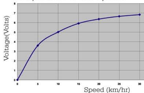
Output of 2.4 W Hub Dynamo
