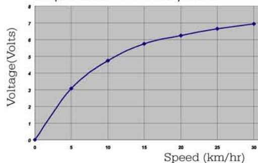
Output of 3.0 W Hub Dynamo
