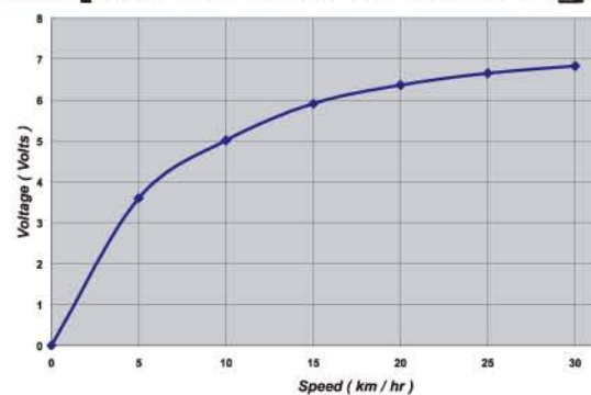
Output of 2.4 W Hub Dynamo
