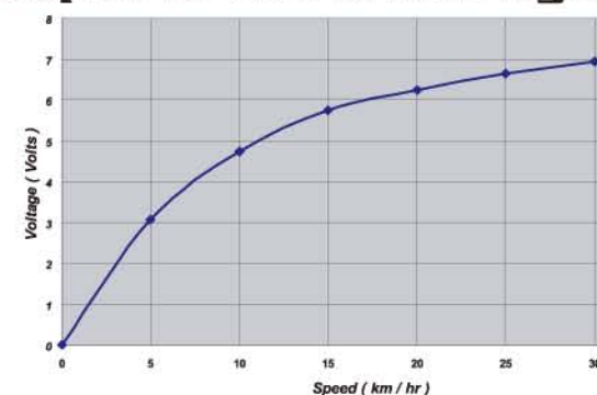
Output of 3.0 W Hub Dynamo
